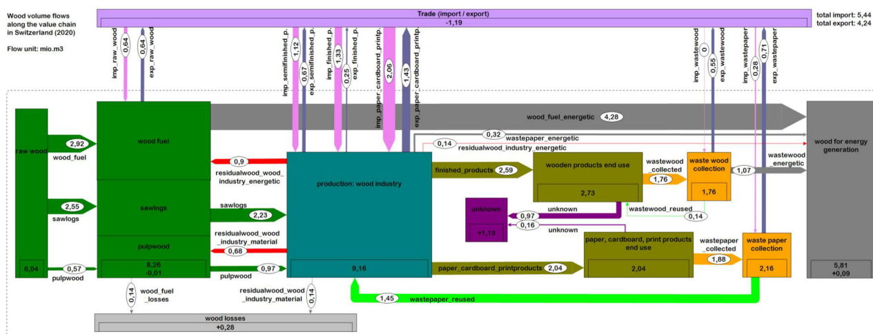
FIGURE 4 Summarized overview of the material flow analysis of wood use along the value chain in Switzerland for the year 2020 in mio.m 3 . The colors represent raw material (green), semifinished products (teal), finished products (olive green), waste wood (orange), wood for energy (dark gray), wood losses (light gray), waste reused (bright green), residual wood (red); unknown (dark violet), import (pink), and export (lavender) (see SI A). The "unknown" flow can be interpreted as a stock increase in society.
